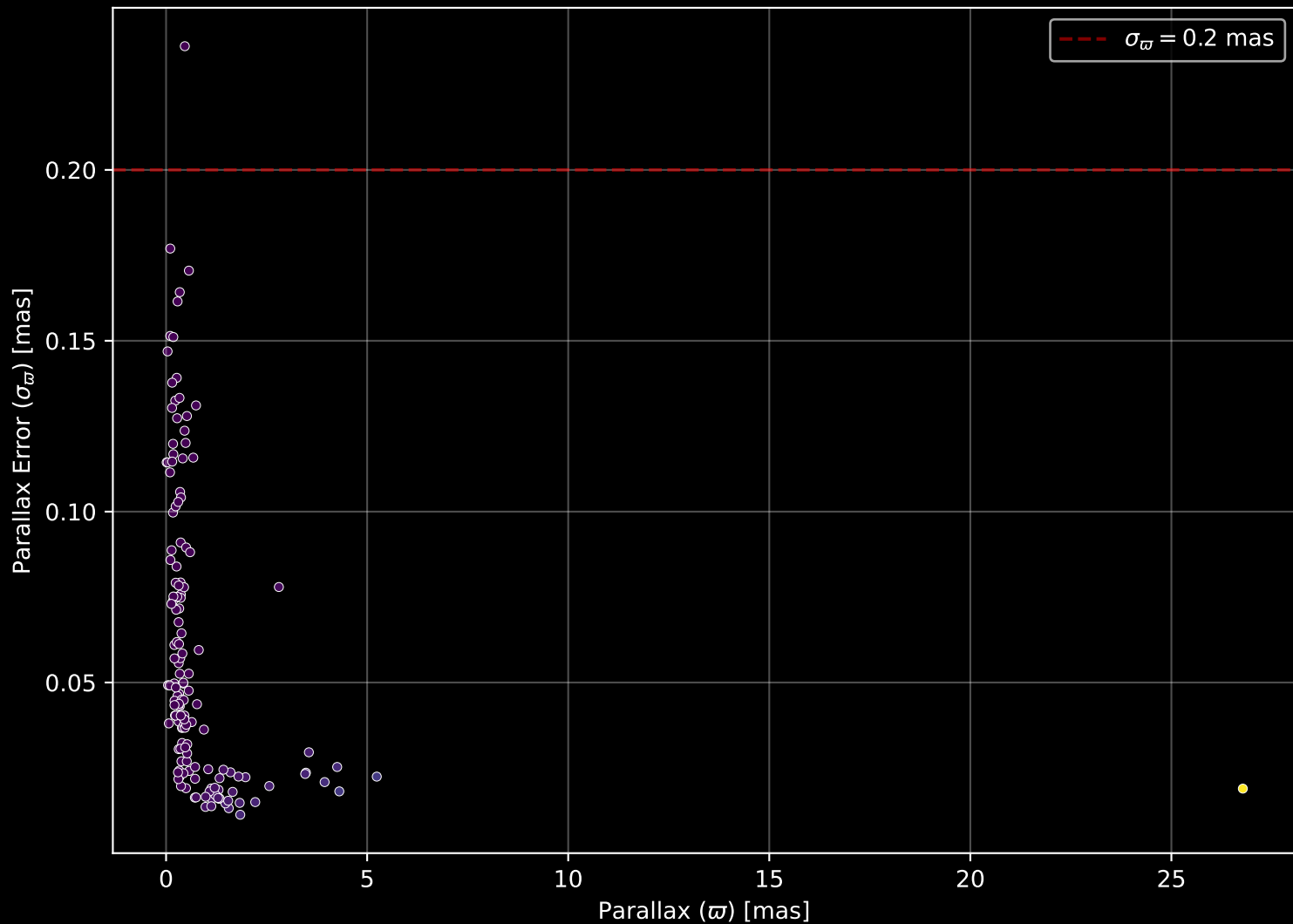
APOGEE DR17 Field: [143+00] Parallax Quality (n= 152)
