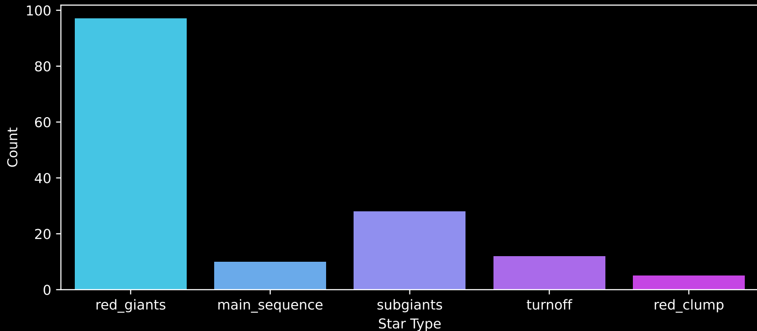
APOGEE DR17 Field: [143+00] Count plot of Star Type
