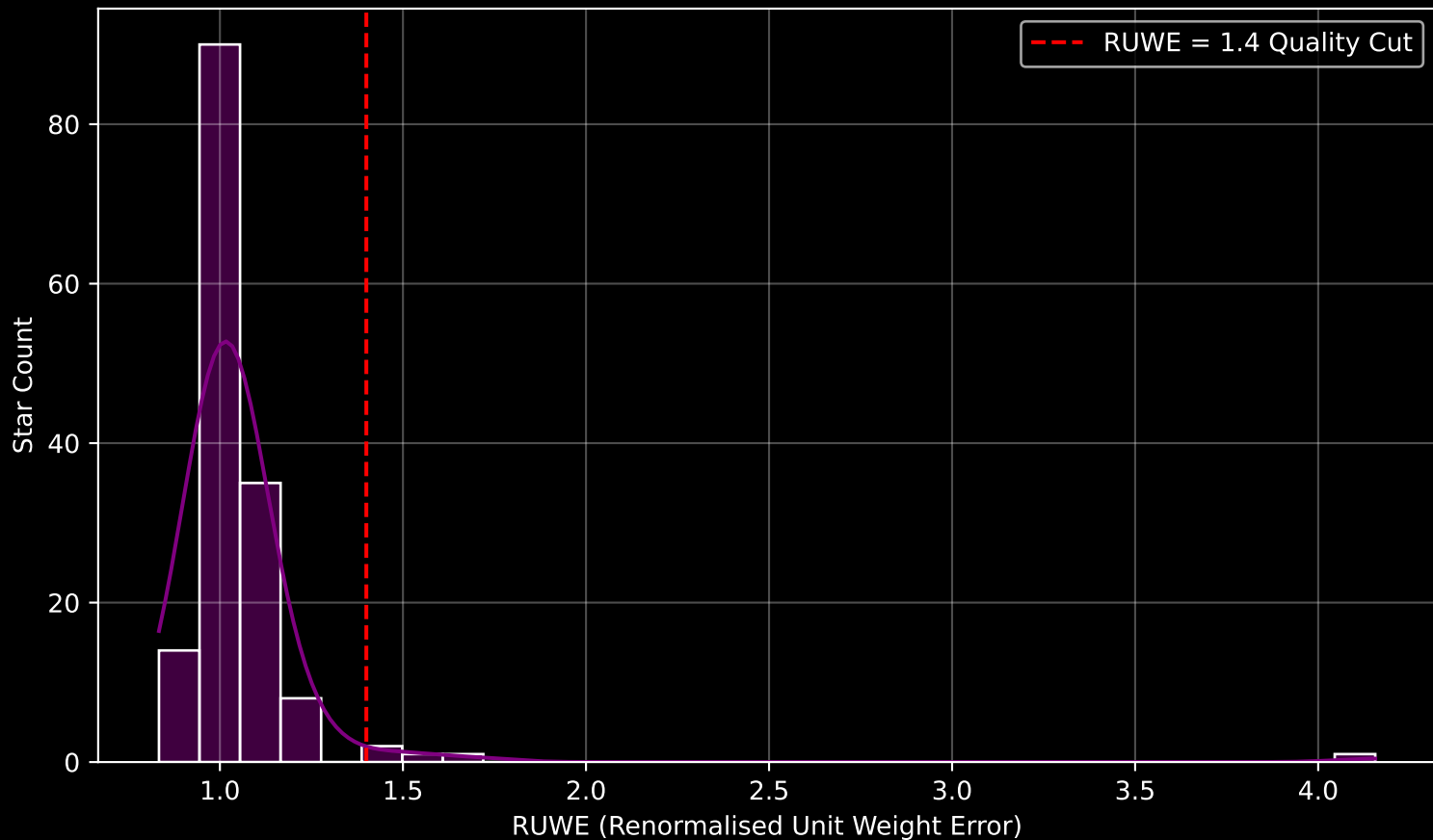
GAPOGEE DR17 Field [143+00] RUWE Distribution (n= 152)
