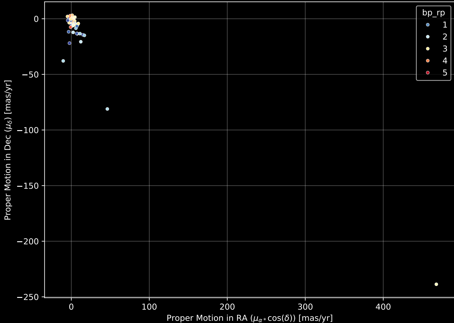
APOGEE DR17 Field: [143+00] Proper Motion Diagram (n= 152)
