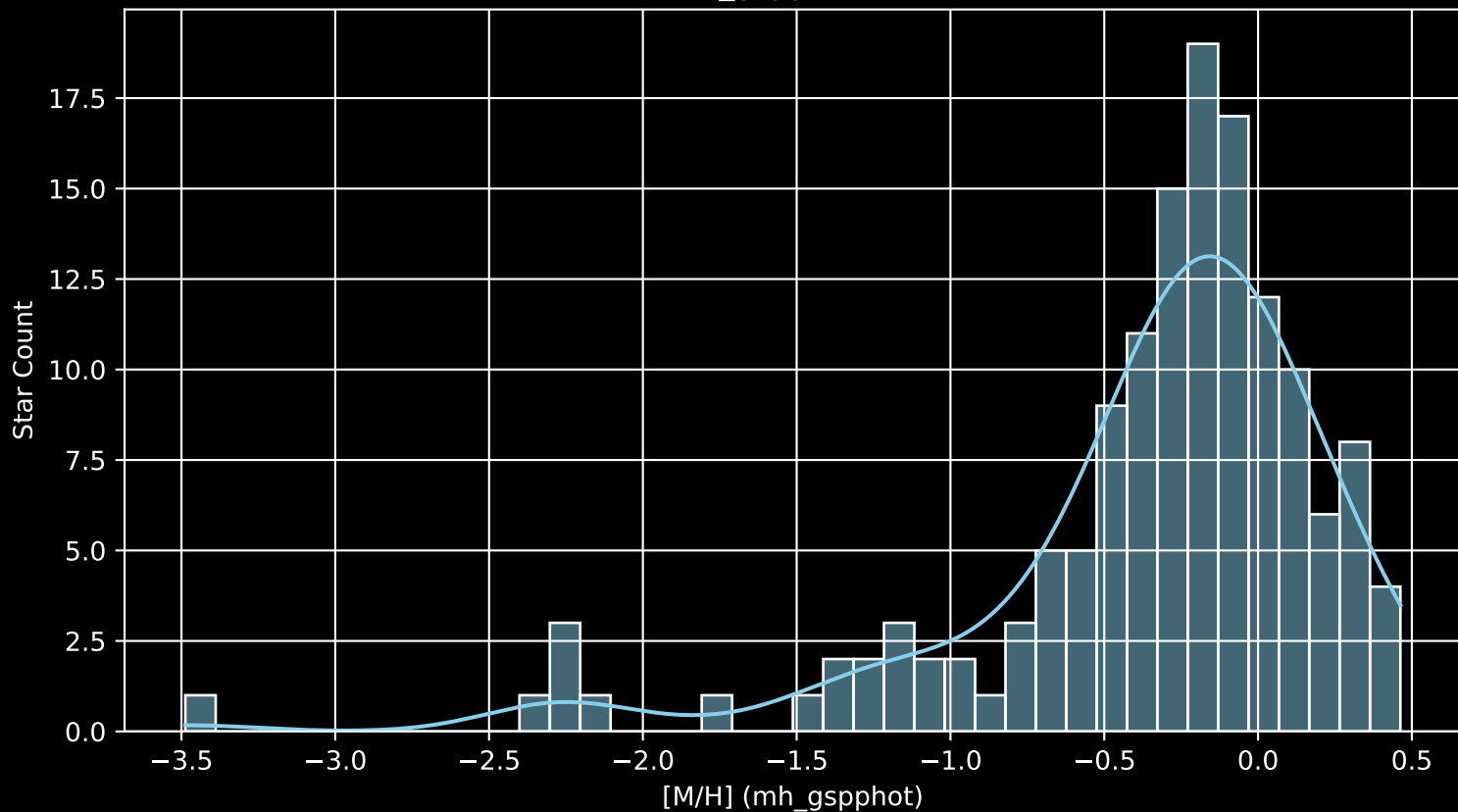
APOGEE DR17 Field: [143+00 [M/H] (mh_gspphot) (n= 144)
